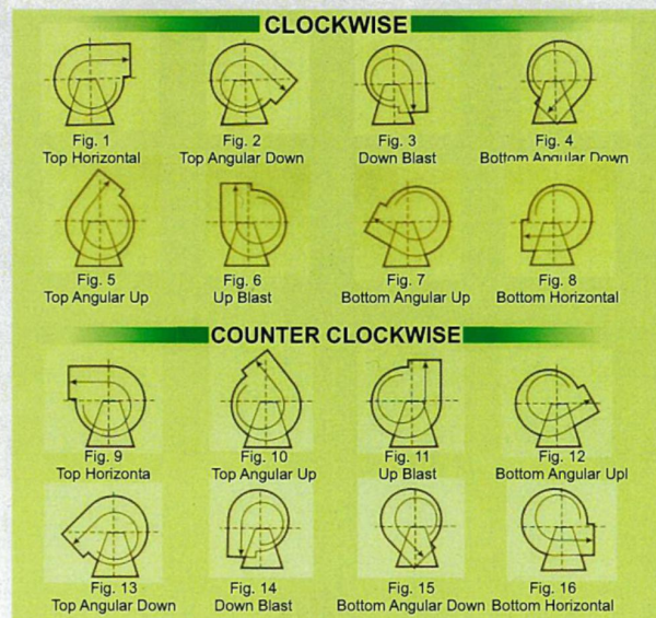
▲ DESIGNATION OF DIRECTION FOR ROTATION AND DISCHARGE
